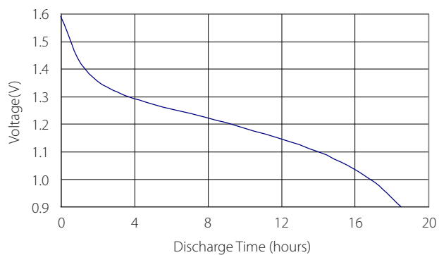
20 \Omega Continuous Discharge Curve
