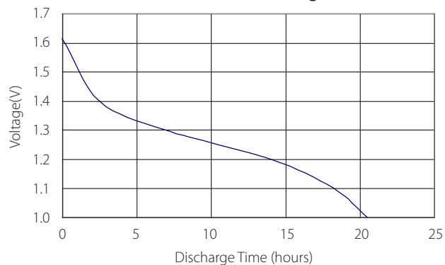
24 \Omega 15s/m-8h/d Discharge Curve
