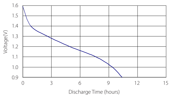
100mA 1h/d Discharge Curve
