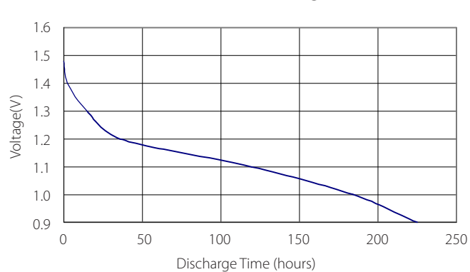
5.1 \Omega 4m/h-8h/d Discharge Curve
