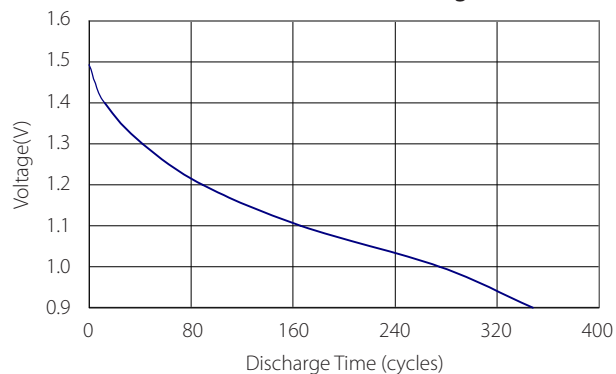
600mA 10s/m, 1h/d Discharge Curve
