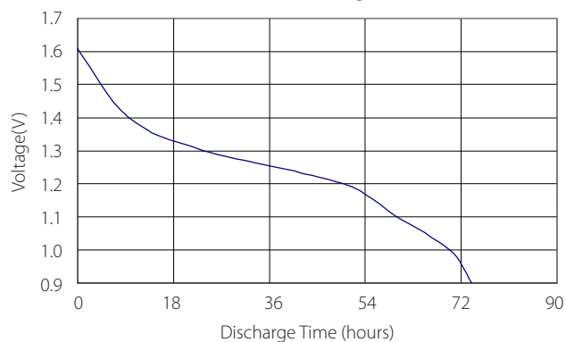
75 \Omega 4h/d Discharge Curve
