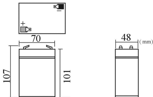
Dimensions(mm) Standard Cover
