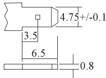
F1(Faston Tab No.187E) Standard Terminal
