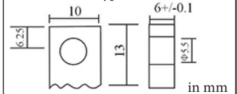
Optional Terminal B2(lead) Bolt Type: M5
